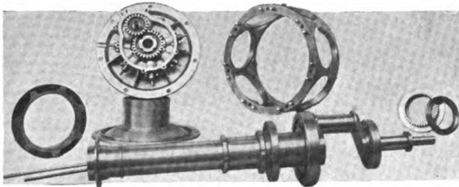
Crankshaft and Details of Gnome 7-Cylinder Motor.
